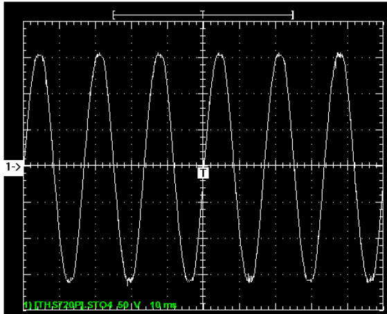
RMS Voltage, 115.5 VAC
