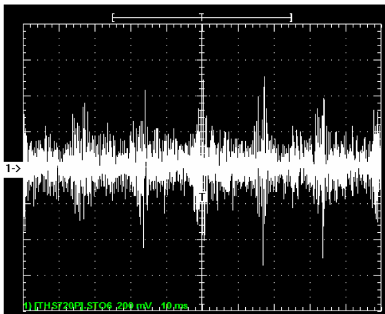
Common Mode Noise, 1.06 V Pk to Pk
